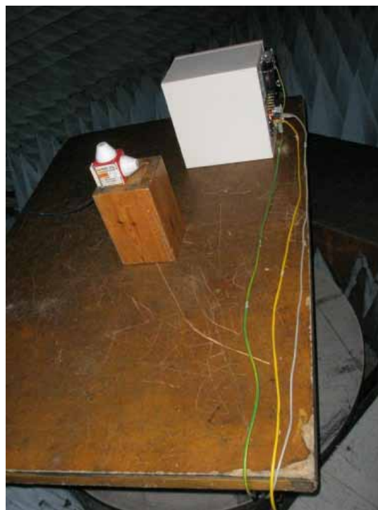
Photograph 8.1.2 Setup for radiated immunity to RF electromagnetic field test, EUT close view, EUT radiation through cable
