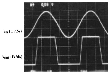
Figure 57. A \pm 7.5V Input Signal Greatly Exceeds the 3V Supply in Figure 58 Causing No Phase Inversion Due to R_I
