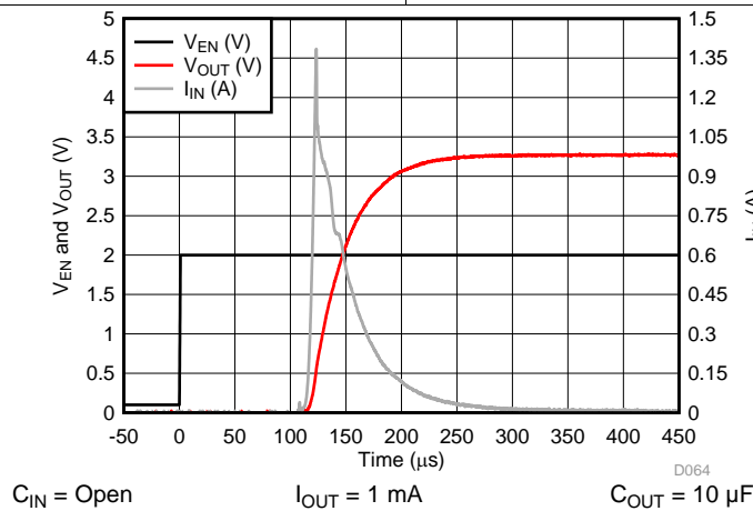
Figure 51. LP5912-3.3 In-Rush Current
