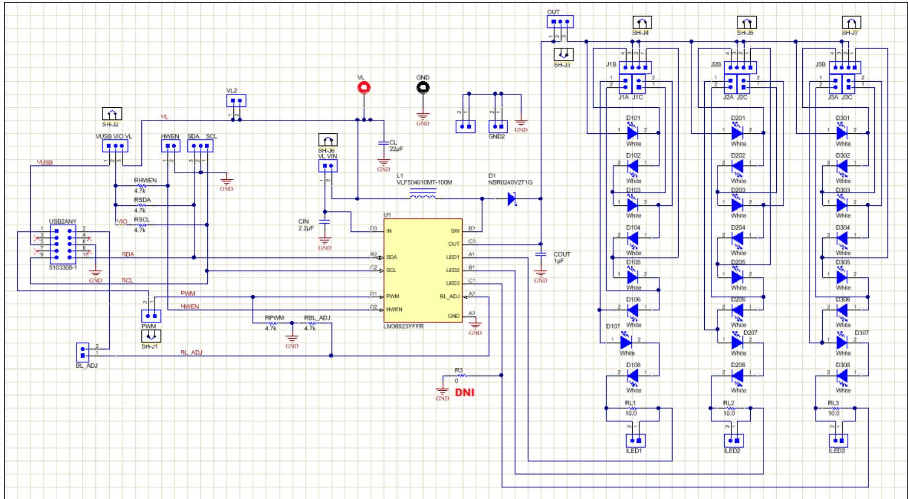
Figure 10. LM36923EVM Schematic
