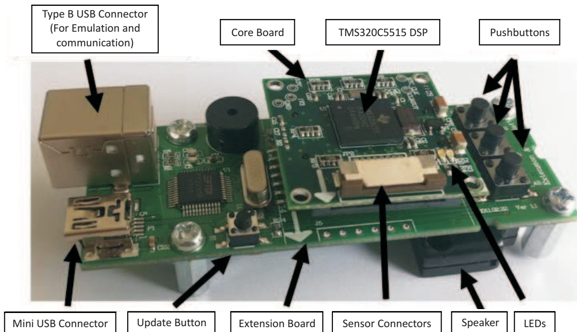
Figure 1. C5515 Fingerprint Development Boards Side View
