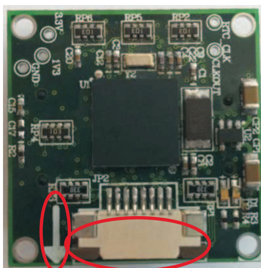
Figure 2. C5515 FDK Core Board
