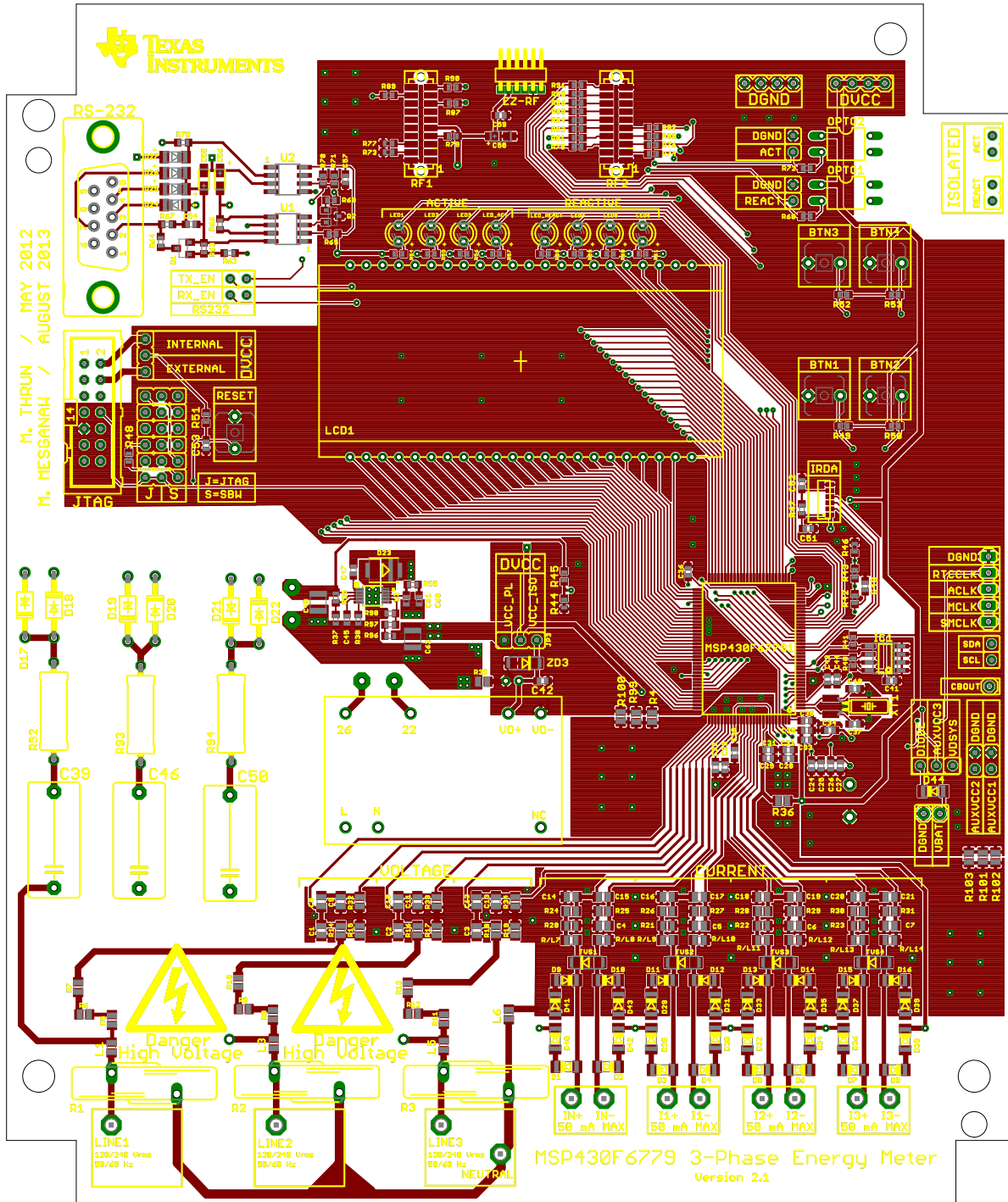
TIDM-THDREADING (EVM430-F6779 TOP LAYER)
