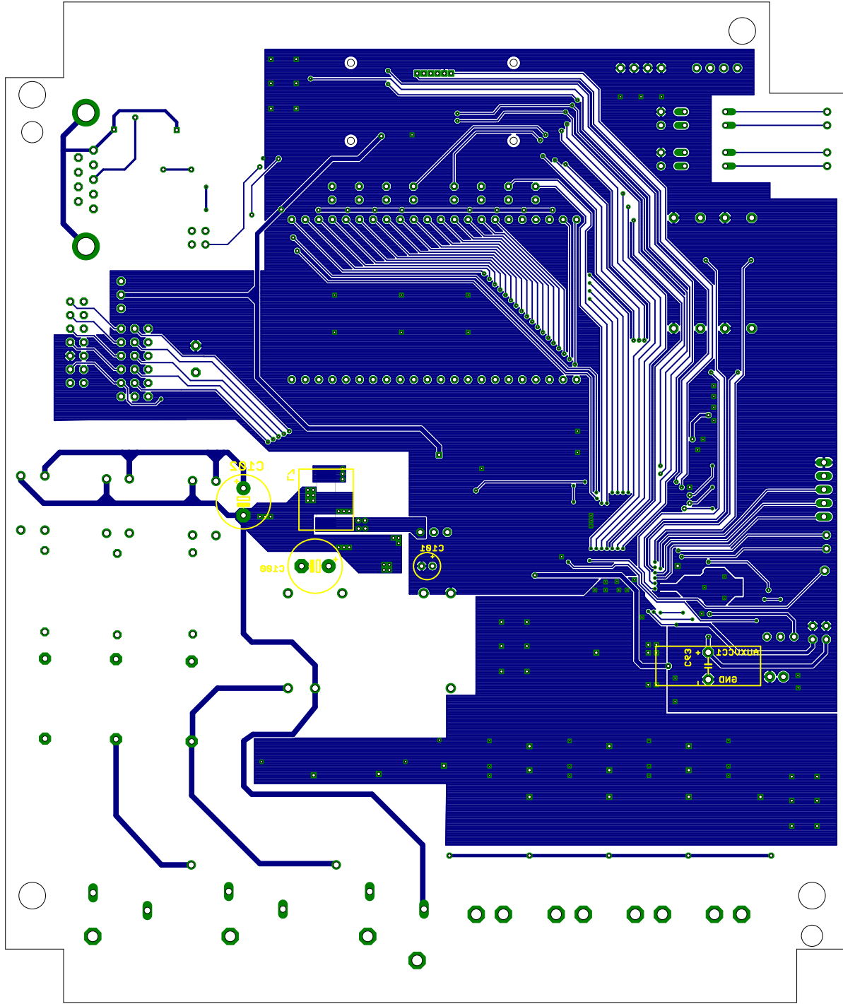
TIDM-THDREADING (EVM430-F6779 BOTTOM LAYER)
