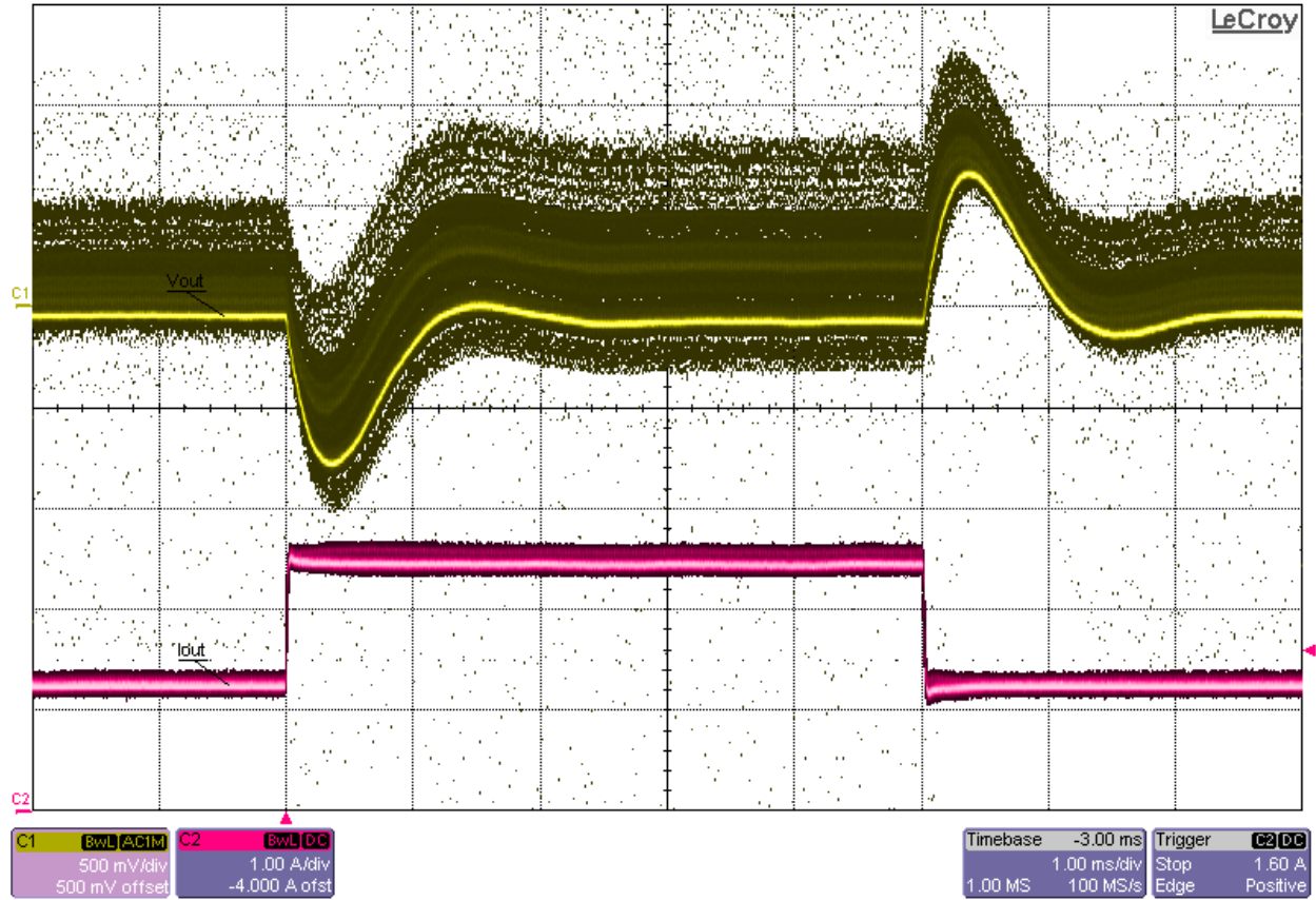
Load Transient Response at 12Vin and 50%-to-100% (1.25A-to-2.5A) Load Step
