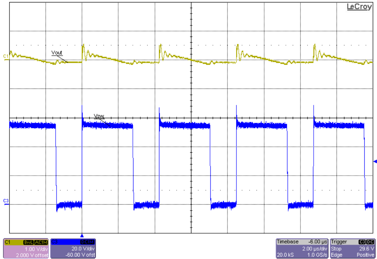
Switch Node Voltage and Output Voltage Ripple at 36Vin and Full (2.5A) Load (Vripple \approx 750mVp-p)
