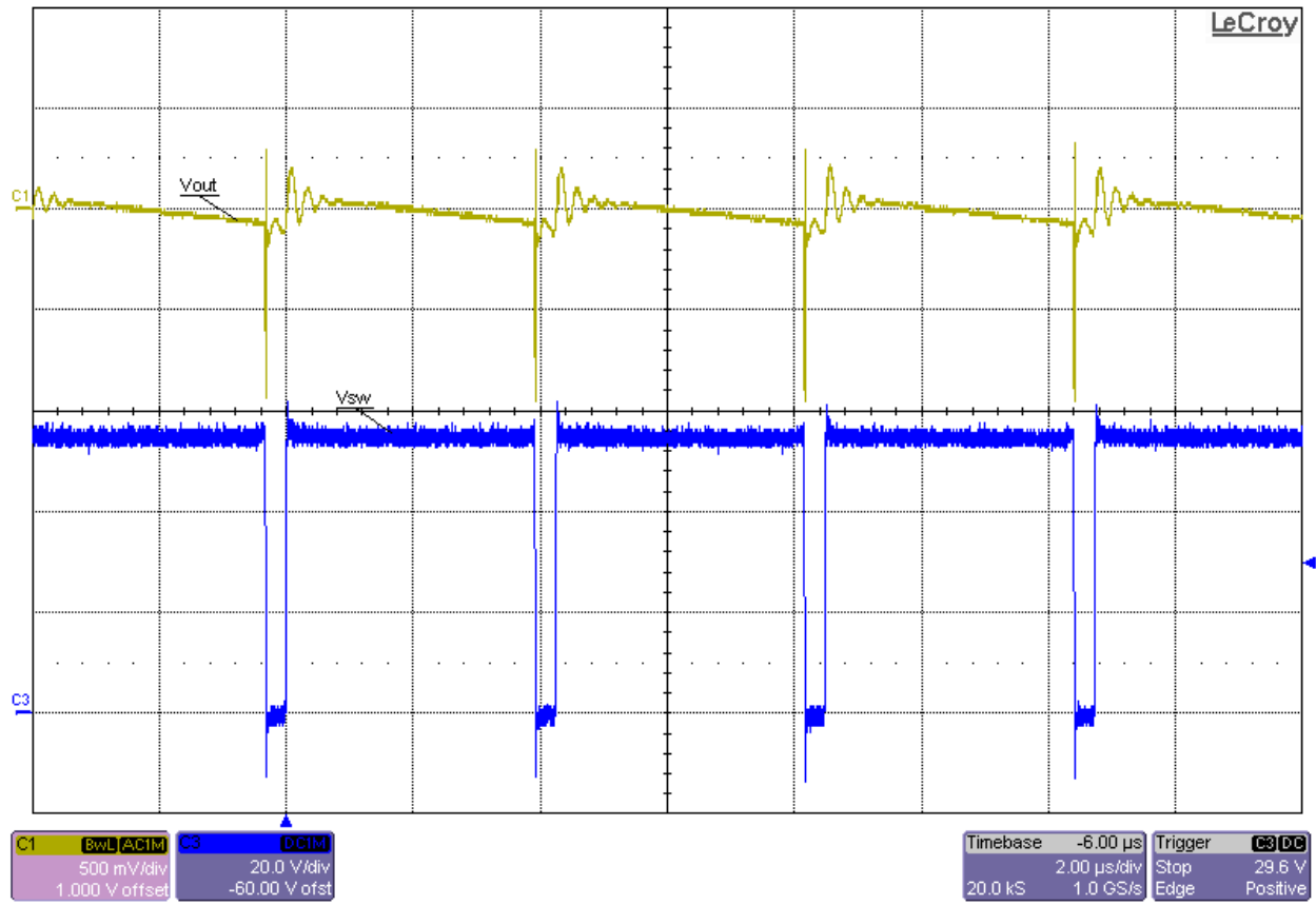
Switch Node Voltage and Output Voltage Ripple at 50Vin and Full (2.5A) Load (Vripple ≈ 350mVp-p)
