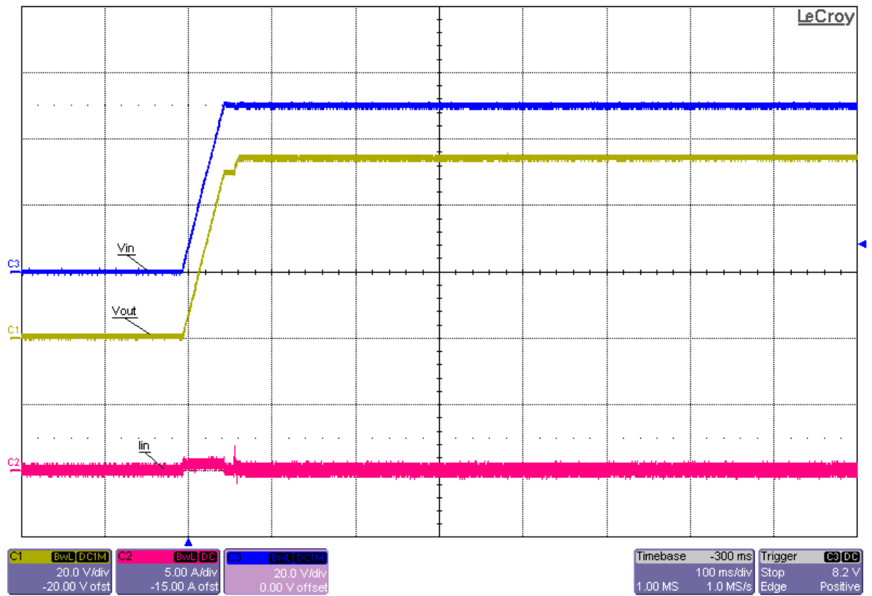
Startup into No Load at 50Vin
