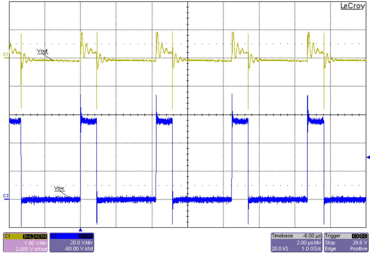
Switch Node Voltage and Output Voltage Ripple at 12Vin and Full (2.5A) Load (Vripple \approx 1.2Vp-p)
