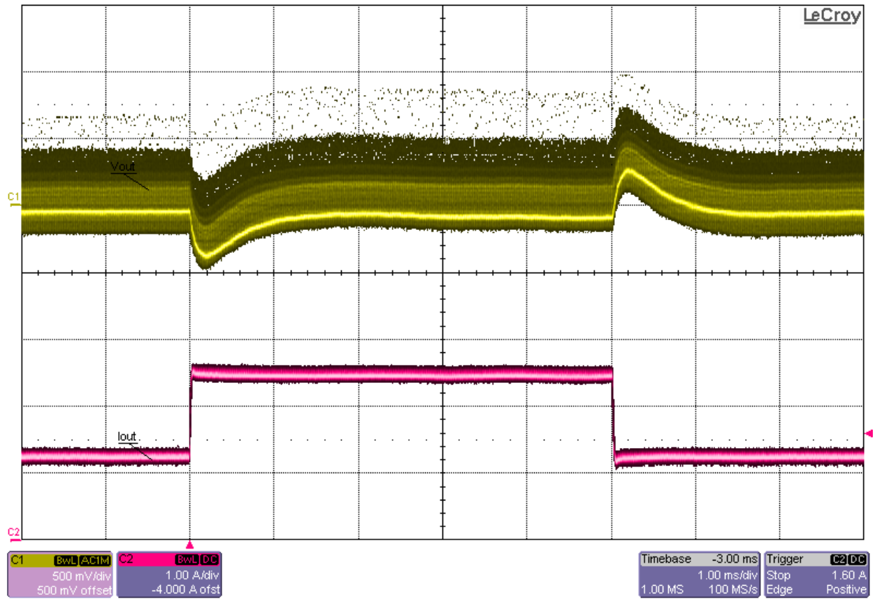
Load Transient Response at 36Vin and 50%-to-100% (1.25A-to-2.5A) Load Step
