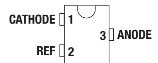
TL431LIA, TL431LIB DBZ 3-Pin, SOT-23 (Top View)
