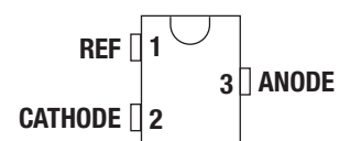
TL432LIA, TL432LIB DBZ 3-Pin, SOT-23 (Top View)
