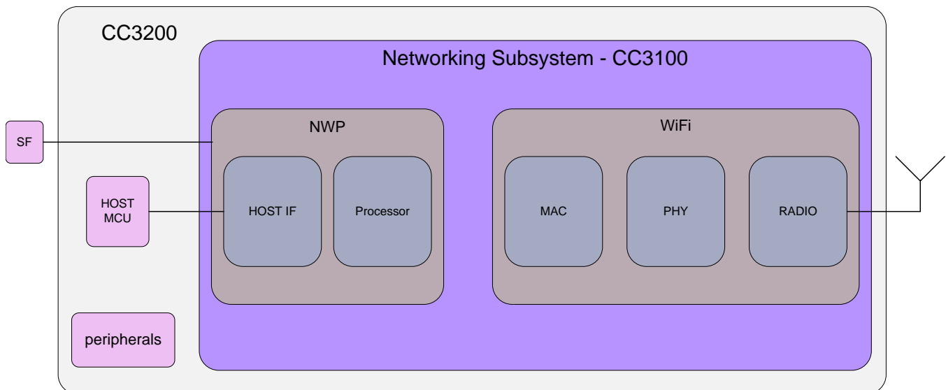
Figure 1. CC3100/CC3200 Block Diagram
