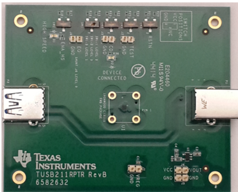
Figure 1. TUSB211RPTREVM Top View
