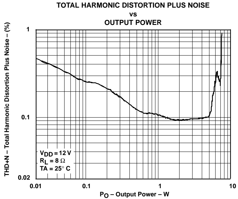
Figure 3–13. Class-D Amplifier Distortion versus Output Power at 8 Ω
