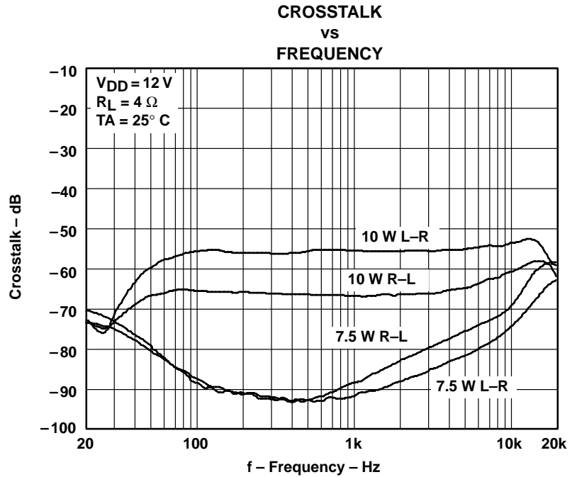
Figure 3–16. Class-D Amplifier Crosstalk versus Frequency Into 4 Ω
