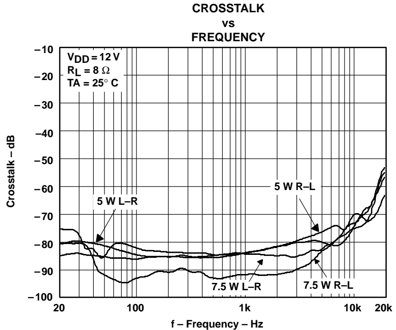
Figure 3–17. Class-D Amplifier Crosstalk versus Frequency Into 8 Ω
