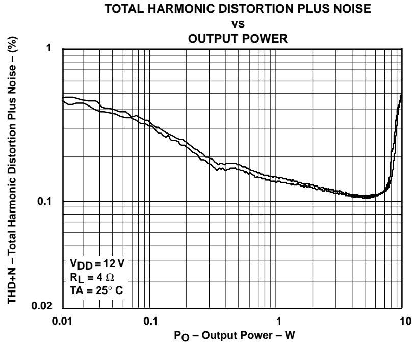
Figure 3–12. Class-D Amplifier Distortion versus Output Power at 4 Ω
