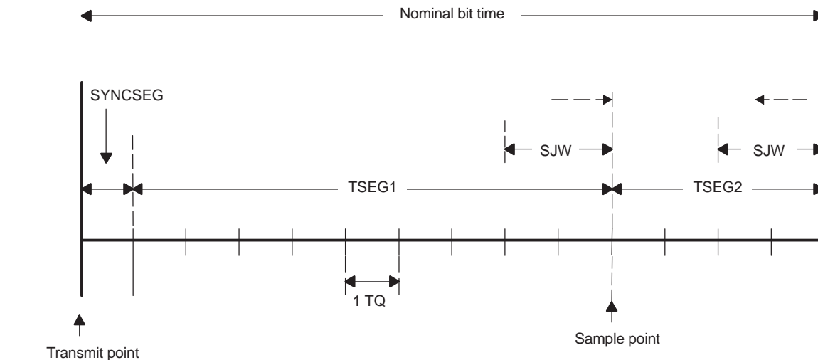
Figure 3-2. CAN Bit Timing
