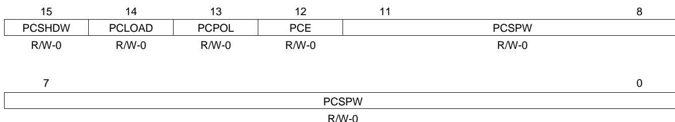
Figure 23. eQEP Position-compare Control (QPOSCTL) Register
