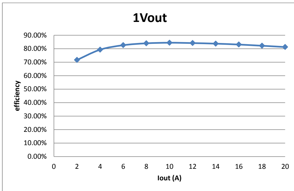
Figure 6. VIN = 12V, VCCINT Efficiency
