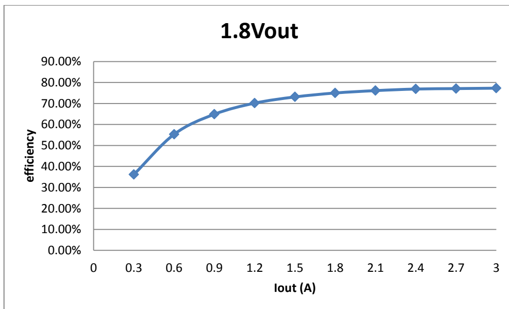
Figure 7. VIN = 12V, VCCAUX Efficiency
