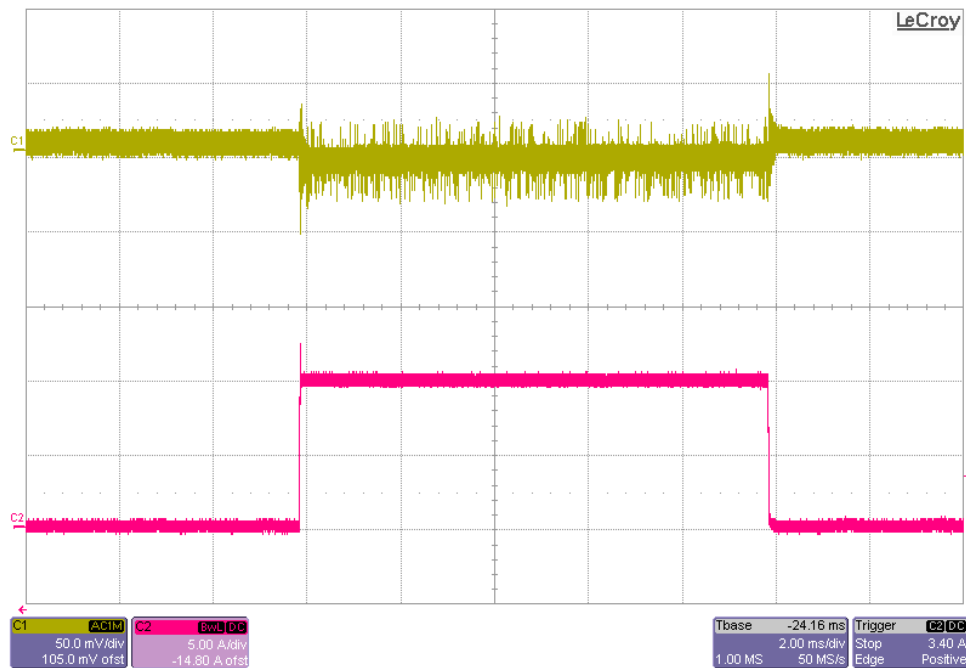
Figure 12. VIN = 12V, VCCINT Load Transient slew rate=1A/us
