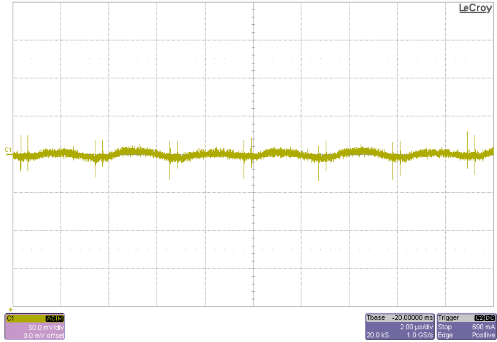
Figure 10. VIN = 12V, VCCINT Output Ripple @ IOOUT = 20A
