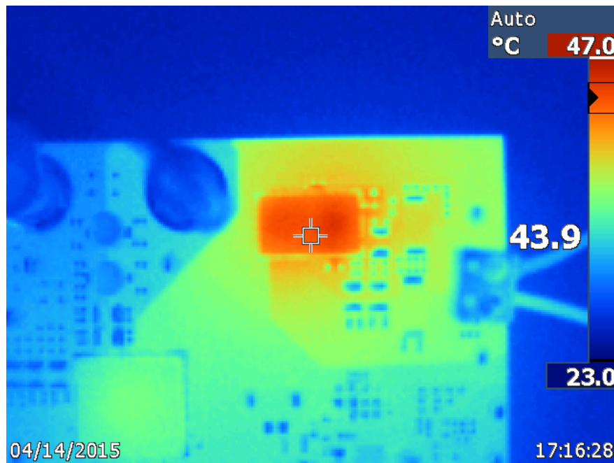
Figure 15. VIN = 12V, VCCAUX Thermal Image @ 3A
