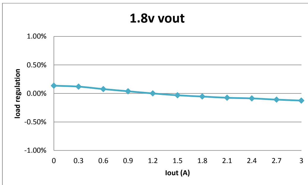
Figure 9. VIN = 12V, VCCAUX Load Regulation
