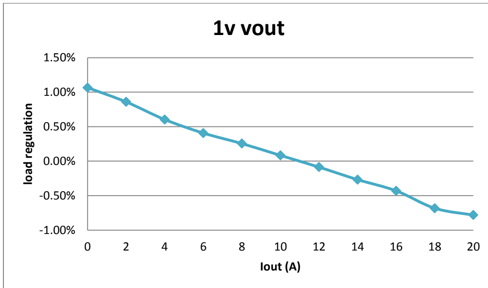
Figure 8. VIN = 12V, VCCINT Load Regulation
