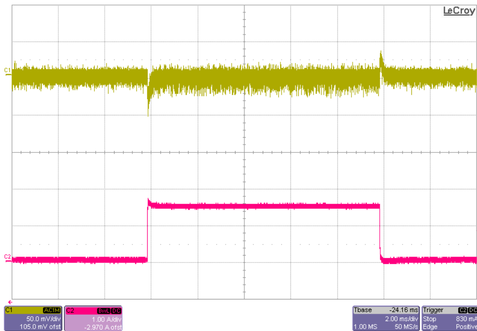
Figure 13. VIN = 12V, VCCAUX Load Transient slew rate=1A/us
