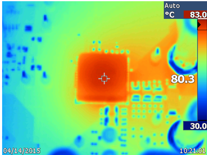
Figure 14. VIN = 12V, VCCINT Thermal Image @ 20A
