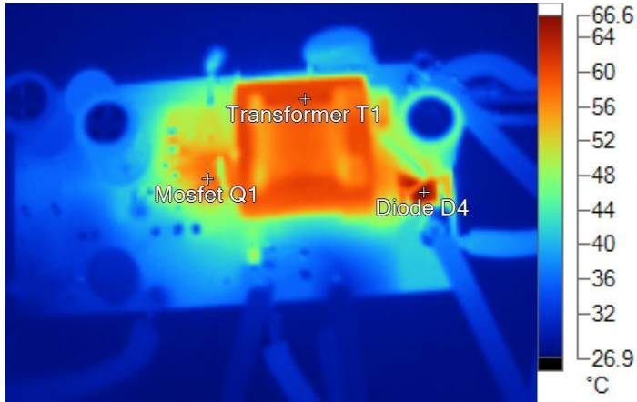
IR20150428_0564 full load Vin=230VAC.is2
