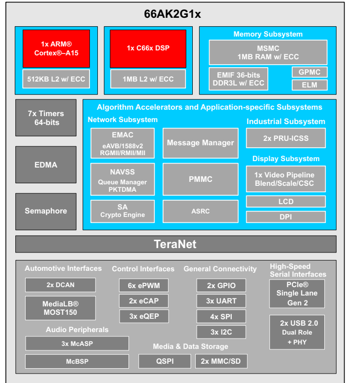
Figure 1: 66AK2Gx processor functional diagram
