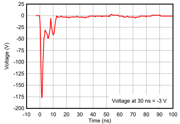
Figure 4-5. -8-kV Clamped IEC Waveform
