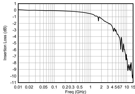
Figure 4-9. Insertion Loss
