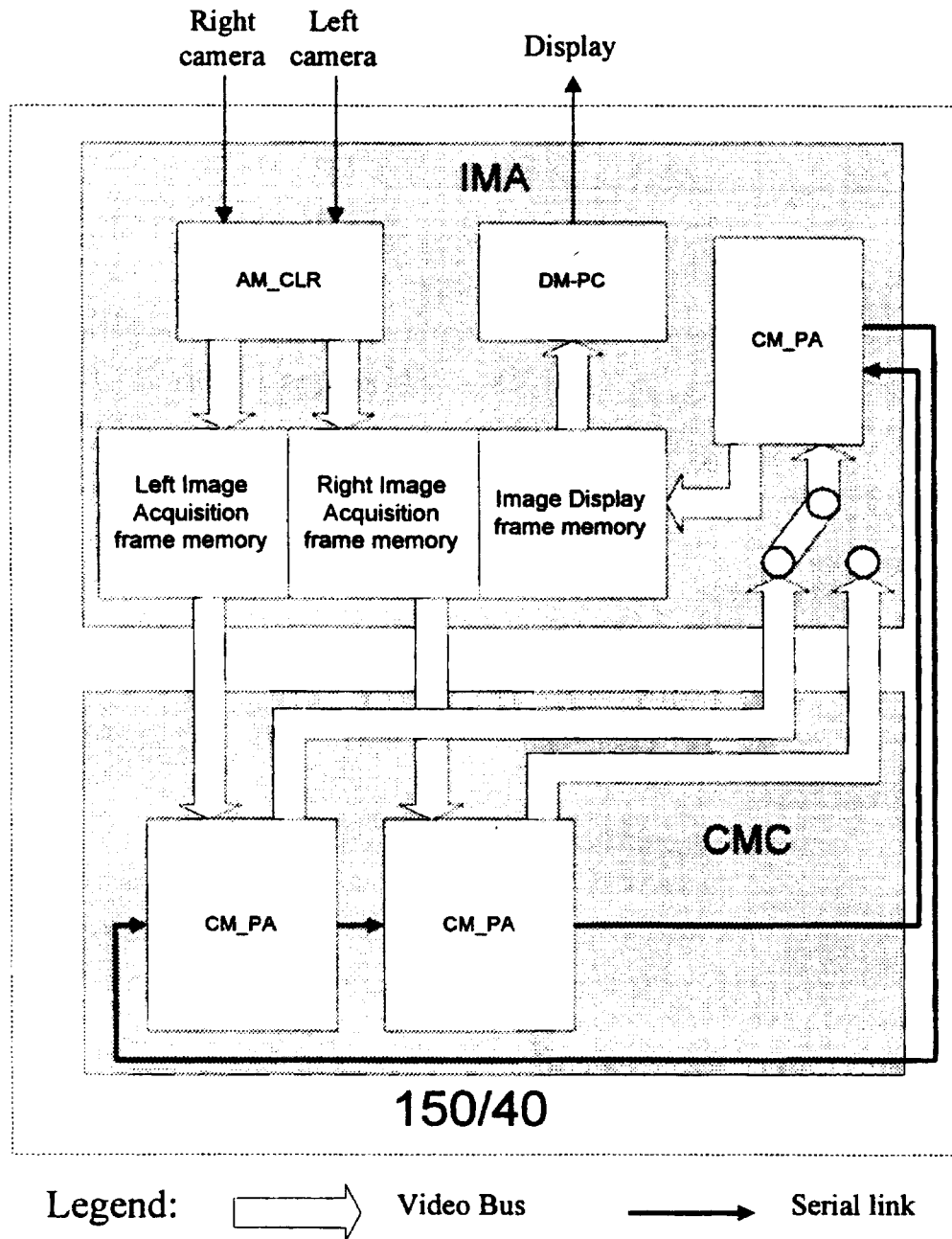
Figure 2. General Configuration
