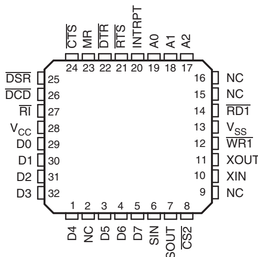
RHB PACKAGE (TOP VIEW)
