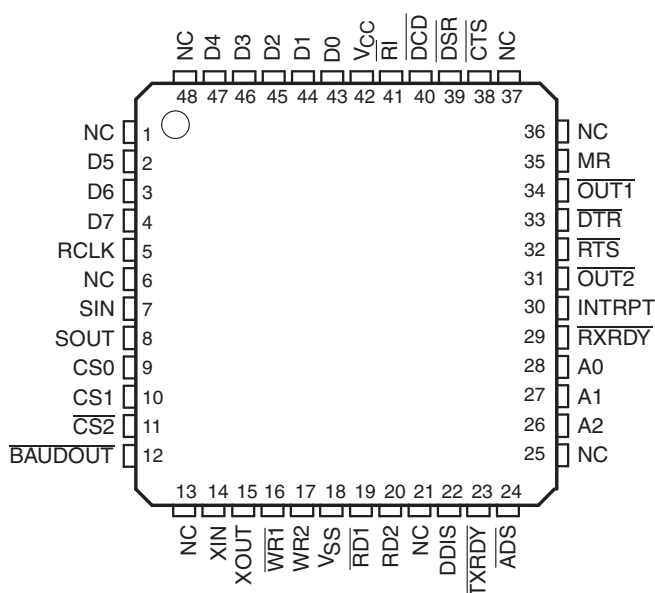
PT/PFB PACKAGE (TOP VIEW)
