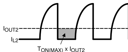
Figure 8-7. Secondary Current Waveforms for C_{OUT2} Ripple Calculation
