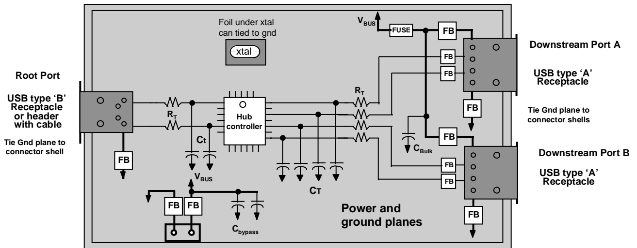
Figure 10: Locally Powered Hub Layout
