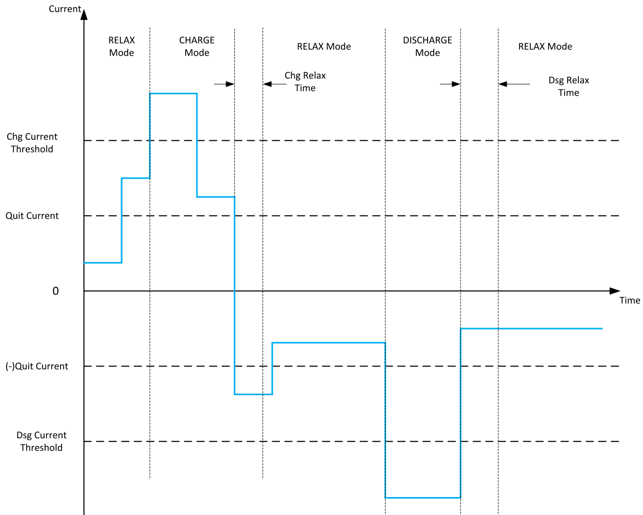
Figure 6-2. Gas Gauge Operating Mode Example
