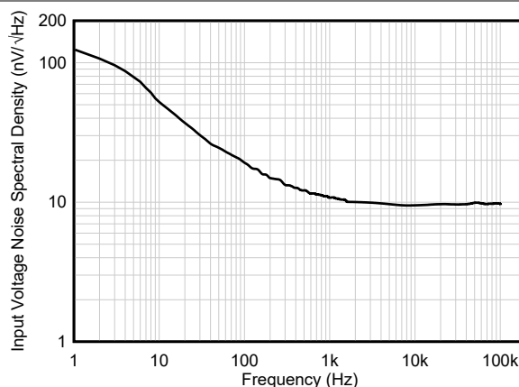
Figure 5-20. Input Voltage Noise Spectral Density vs Frequency
