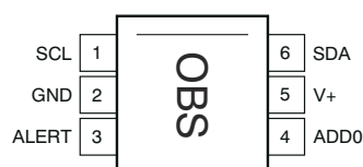
DRL Package 6-Pin SOT563 (Top View)
