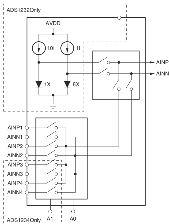
图 7-1. Measurement of the Temperature Sensor in the Input Multiplexer
