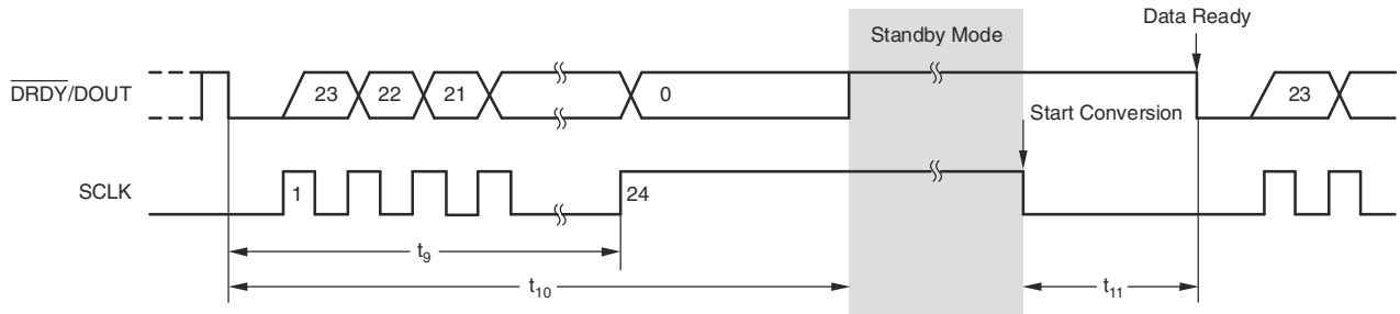
图 7-12. Standby Mode Timing (Can be Used for Single Conversions)
