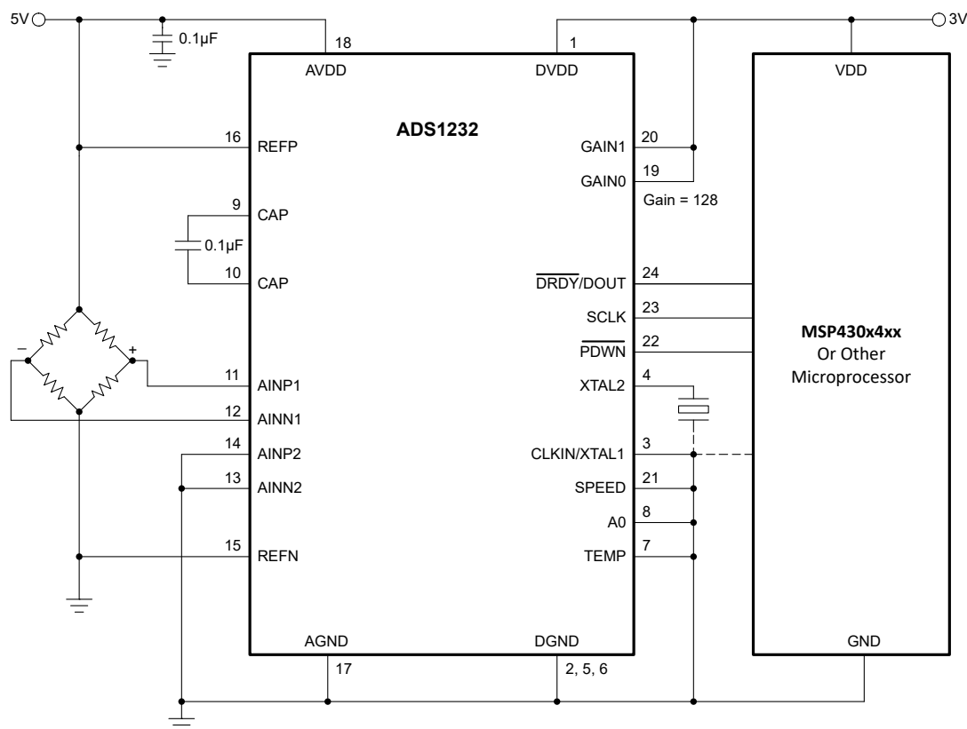
图 8-1. Weigh-Scale Application
