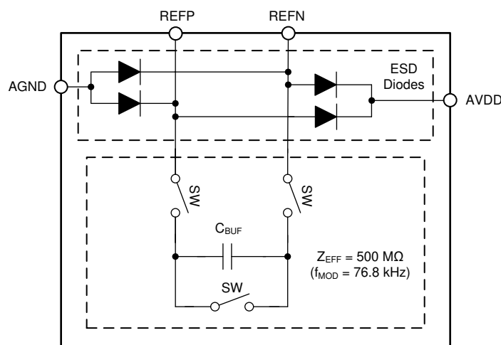
图 7-3. Simplified Reference Input Circuitry
