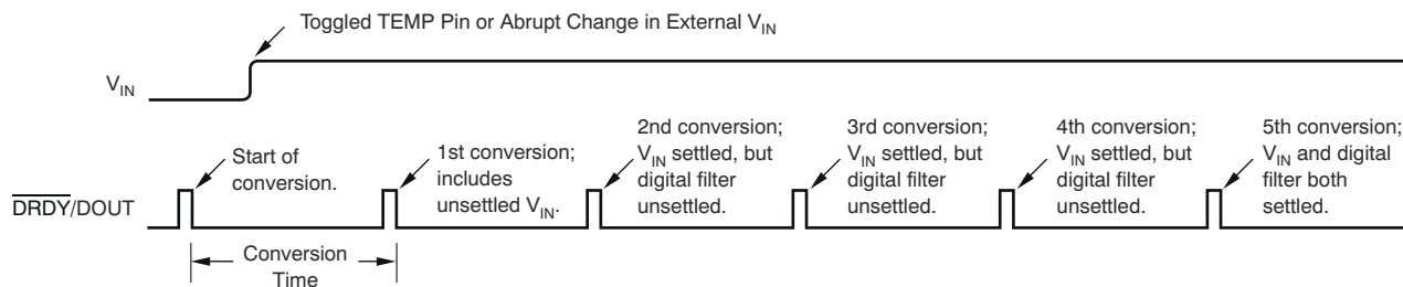
图 7-8. Settling Time in Continuous Conversion Mode
