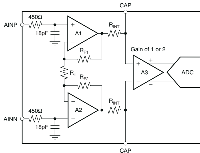
图 7-2. Simplified Diagram of the PGA
