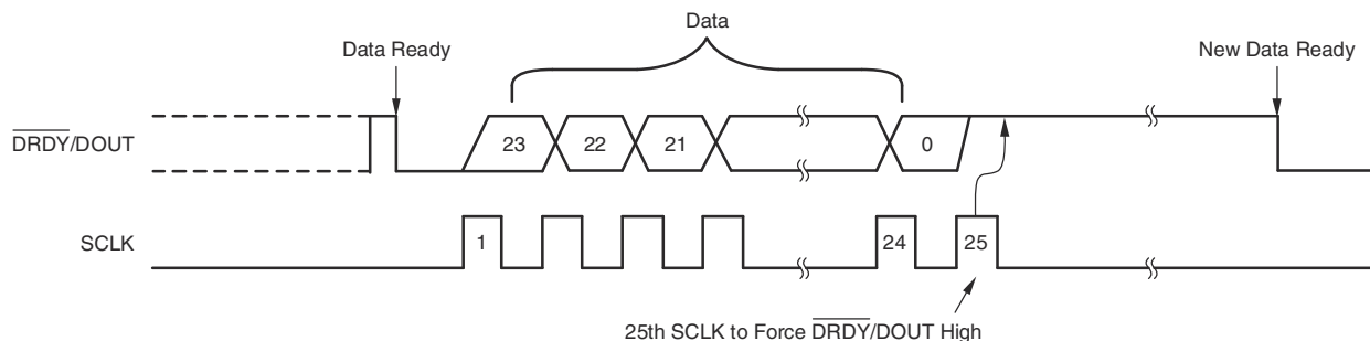
图 7-10. Data Retrieval With \overline{\text{DRDY}}/\text{DOUT} Forced High Afterwards
