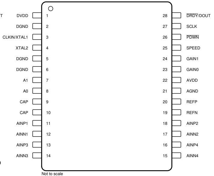
图 4-2. ADS1234 PW Package, 28-Pin TSSOP (Top View)
