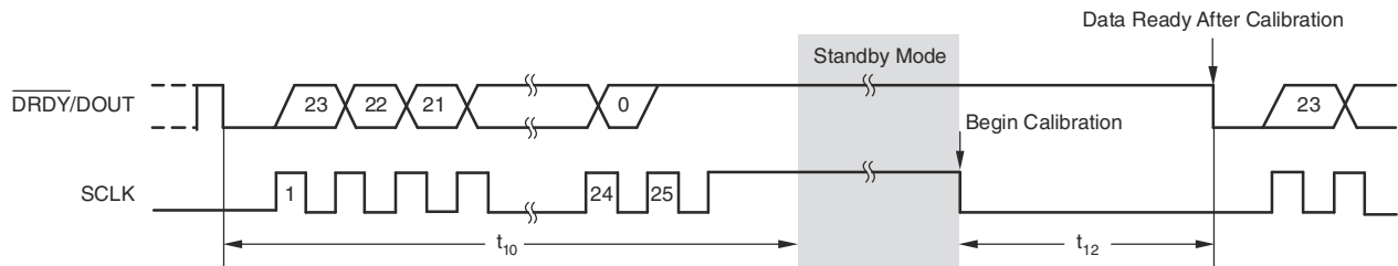
图 7-13. Standby Mode With Offset-Calibration Timing (Can be Used for Single Conversions)
