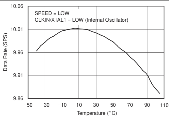
图 5-25. Data Rate vs Temperature
