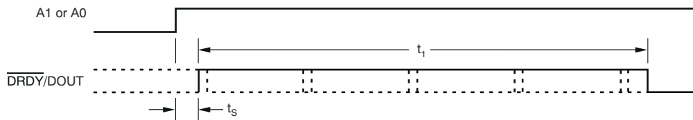
图 7-7. Example of Settling Time After Changing the Input Multiplexer
