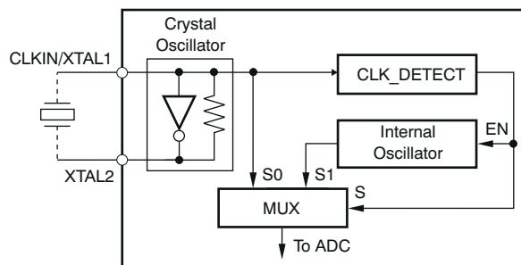
图 7-4. Equivalent Circuitry of the Clock Source
