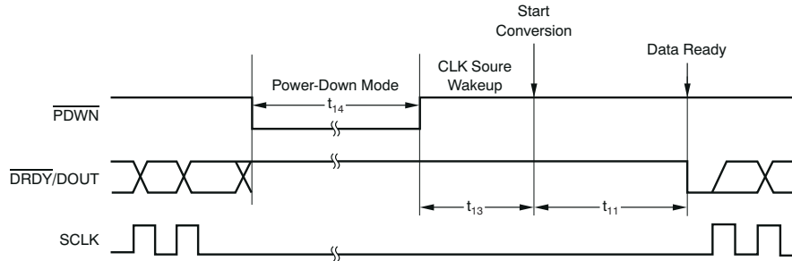
图 7-14. Wake-Up Timing From Power-Down Mode
