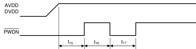
图 7-15. Power-Up Timing Sequence
