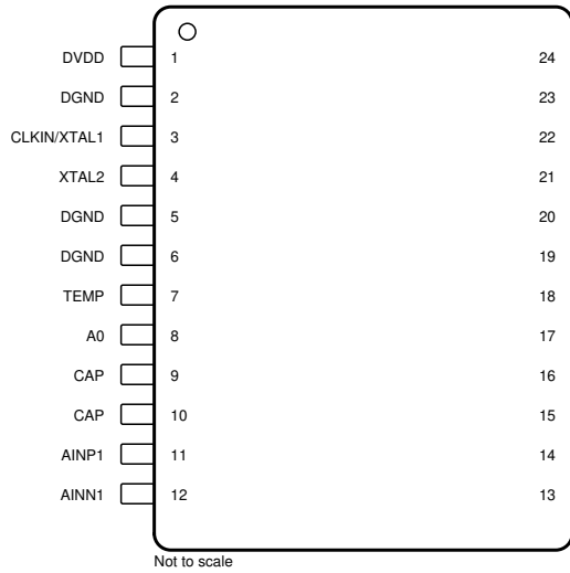
图 4-1. ADS1232 PW Package, 24-Pin TSSOP (Top View)
