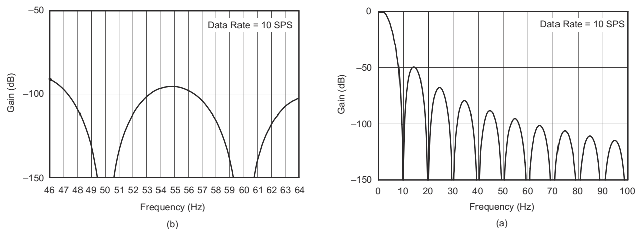
图 7-6. Digital Filter Frequency Response to 100 Hz
