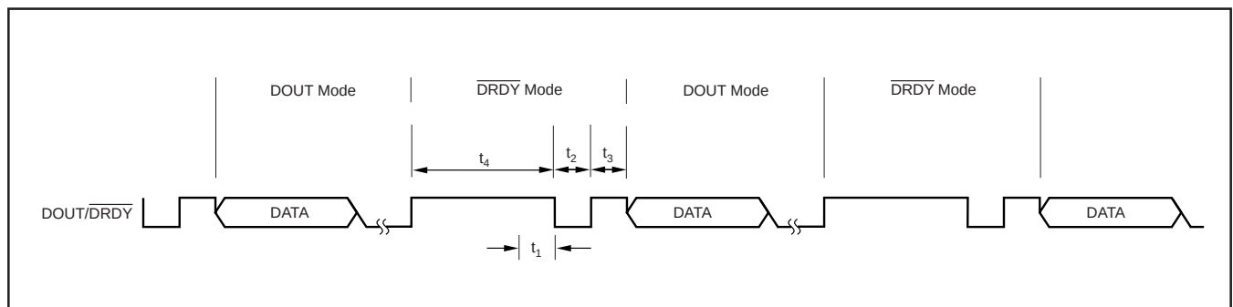
FIGURE 11. DOUT/DRDY Partitioning.
