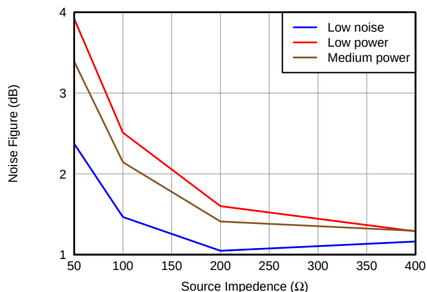
Figure 33. Noise Figure vs. Power Modes without Termination
