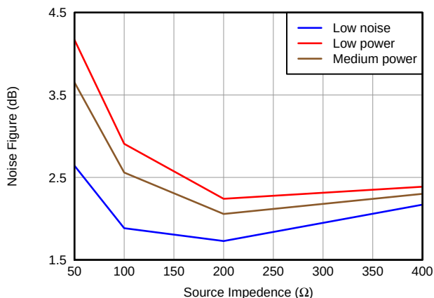
Figure 32. Noise Figure vs. Power Modes with 400 Ω Termination
