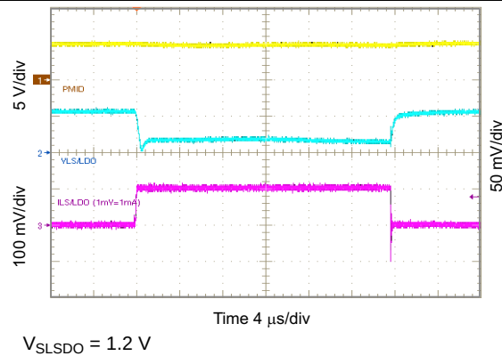
图 87. 1.2 V LSLDO Load Transient, 0 to 100 mA
