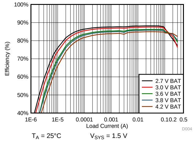
图 45. 1.5 V SYS System Efficiency
