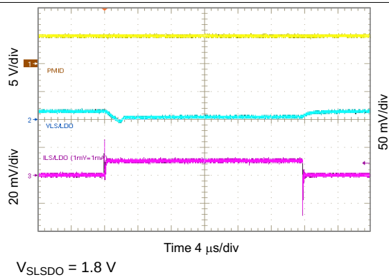
图 83. 1.8 V LSLDO Load Transient, 0 to 10 mA
