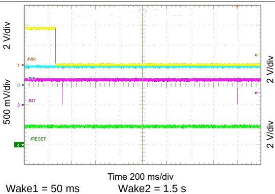
图 98. Show \overline{\text{MR}} Timing
