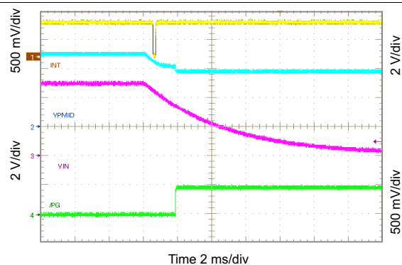
图 94. Show \overline{\text{PG}} and \overline{\text{INT}} Timing ( V_{\text{IN}} Removal)
