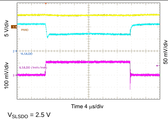
图 89. 2.5 V LSLDO Load Transient, 0 to 100 mA
