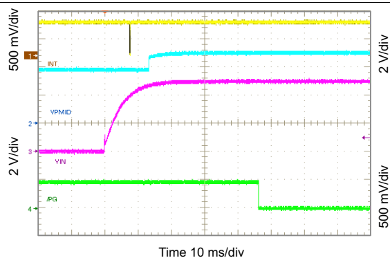
图 93. Show \overline{\text{PG}} and \overline{\text{INT}} Timing ( V_{\text{IN}} Insertion)
