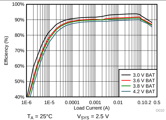
图 47. 2.5 V SYS System Efficiency
