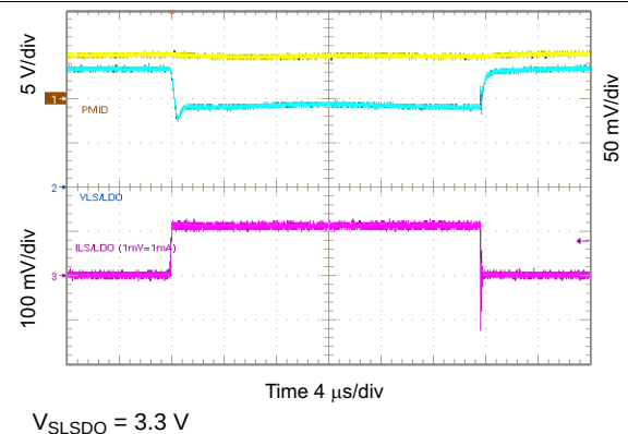
图 90. 3.3 V LSLDO Load Transient, 0 to 100 mA
