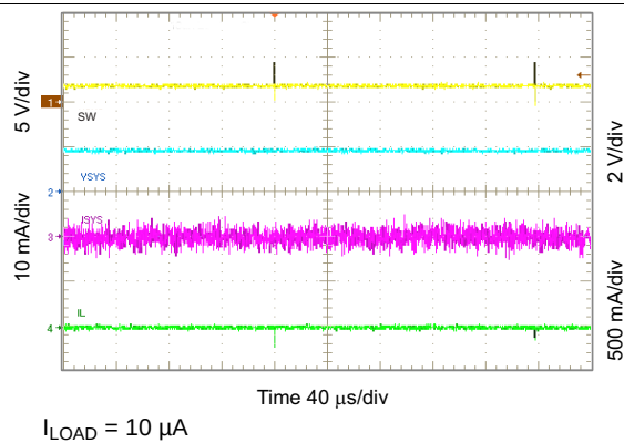
图 60. Light Load Operation Showing SW
