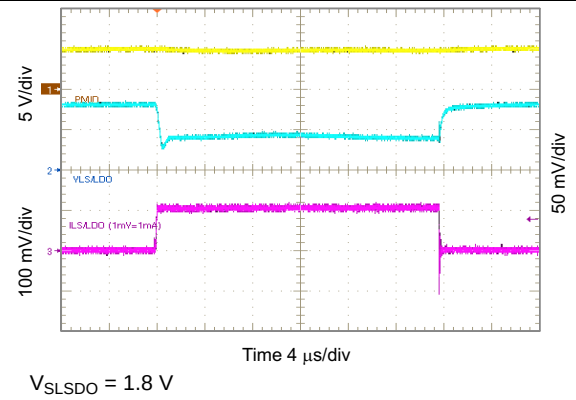
图 88. 1.8 V LSLDO Load Transient, 0 to 100 mA
