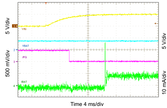
图 37. Power Supply Connected to V_{IN}
