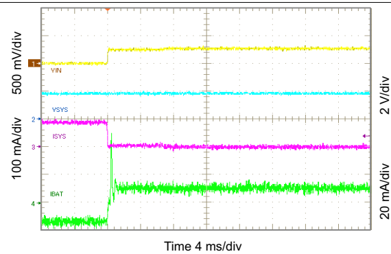
图 41. Exiting Battery Supplement Mode
