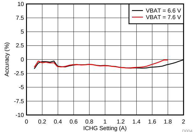
图 8. Charge Current Accuracy vs. ICHG Setting
