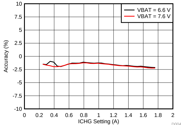
图 7. Charge Current Accuracy vs. ICHG Setting
