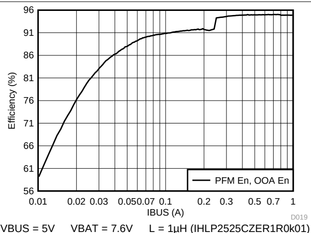
图 6. OTG Efficiency vs. VBUS Output Current
