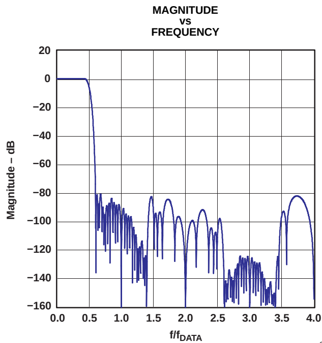
Figure 41. Magnitude Spectrum for 8× Interpolation (dB)
