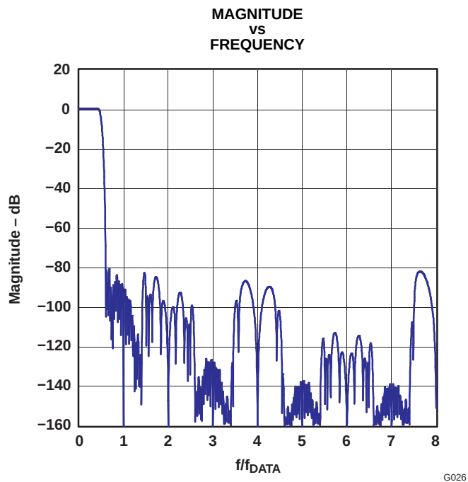
Figure 42. Magnitude Spectrum for 16× Interpolation (dB)
