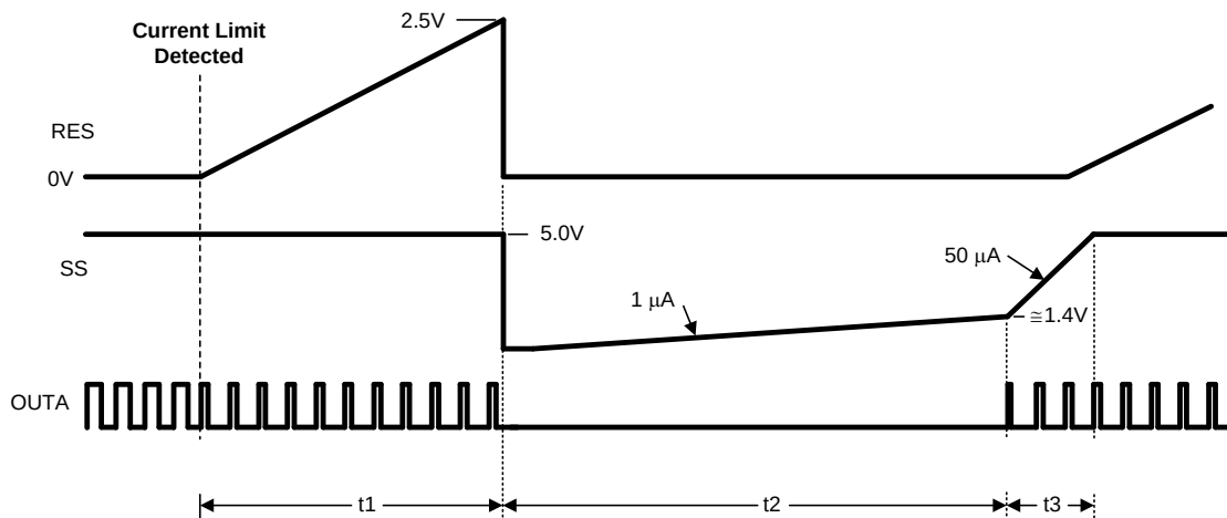
Figure 19. Hiccup Overload Restart Timing
