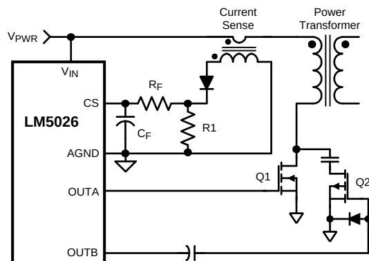
Figure 28. Current Sense Using a Current-Sense Transformer
