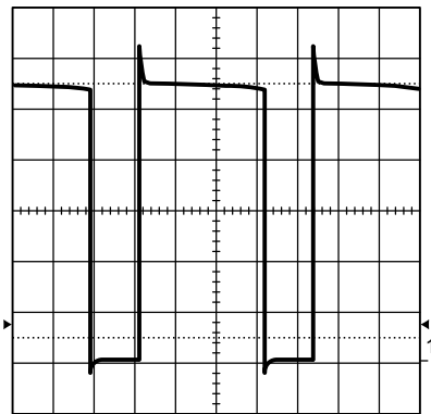
Figure 34. Typical Output Ripple
