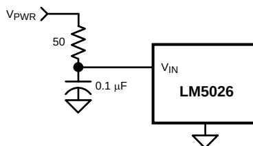
Figure 24. Input Transient Protection
