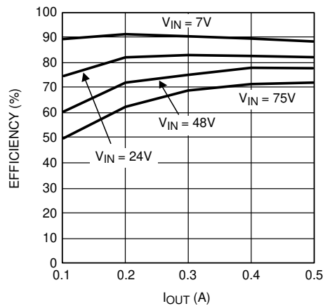
图 5-7. Demoboard Efficiency vs I_{OUT} and V_{IN}
