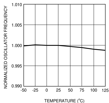
图 5-2. Oscillator Frequency vs Temperature F_{OSC} = 200\text{kHz}
