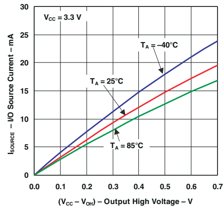
图 5-8. I/O Source Current vs Output High Voltage (P7 - P1)
