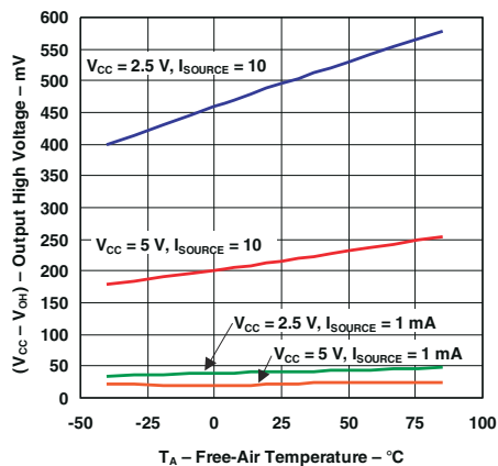
图 5-11. Output High Voltage vs Temperature (P7 - P1)
