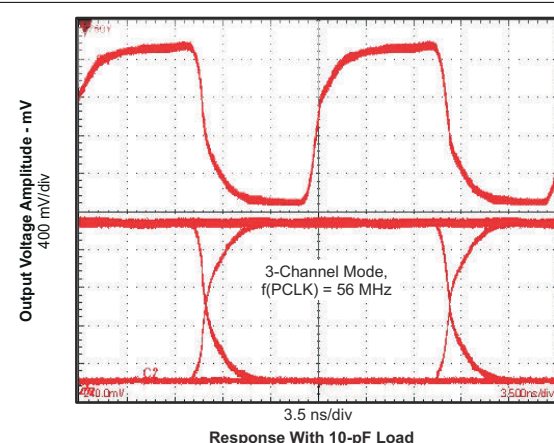
图 6-17. XGA 3-channel Output Waveform on the SN65LVDS302 when driven by the SN65LVDS301
