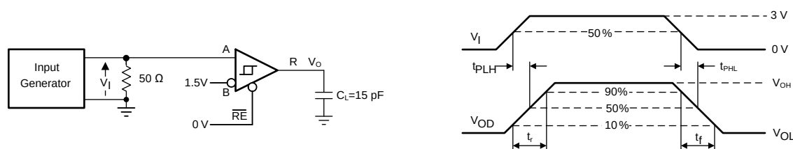
图 16. Measurement of Receiver Output Rise and Fall Times and Propagation Delays
