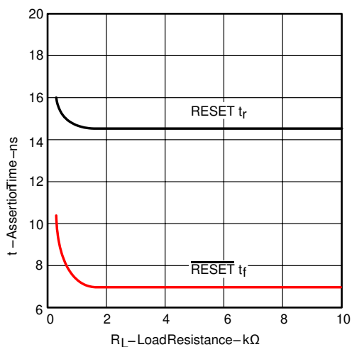
图 6-3. Assertion Time vs Load Resistance
