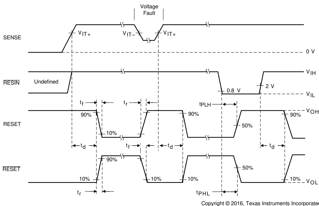
图 8-1. TL77xxB RESET and \overline{\text{RESET}} Response and Timing
