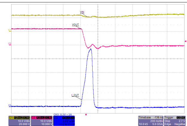
Figure 32. Transient: Recovery from Short Circuit
