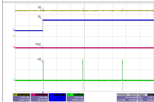
Figure 33. Transient: Output Short Circuit
