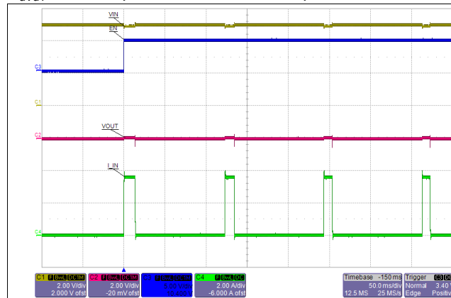
Figure 31. Transient: Wake Up to Short Circuit
