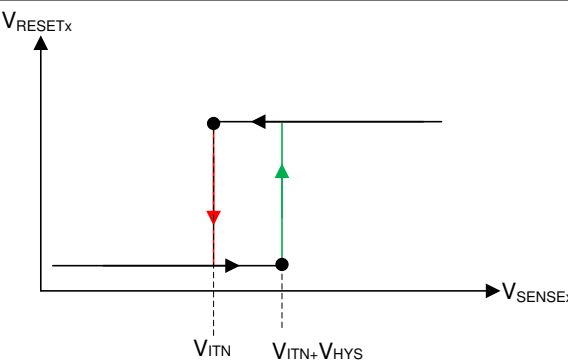
图 8-7. Hysteresis (Undervoltage Active-Low)
