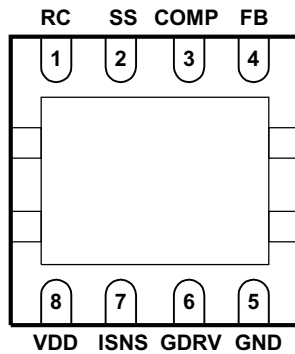
8 PINS VSON (DRB) PACKAGE (BOTTOM VIEW)
