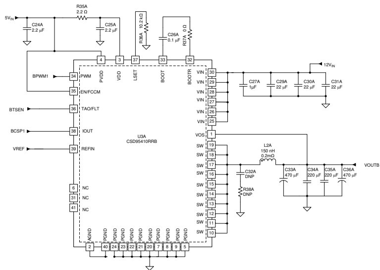
图 8-3. Powerstages Schematic (2/2)
