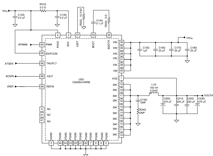
图 8-3. Powerstages Schematic (2/2)
