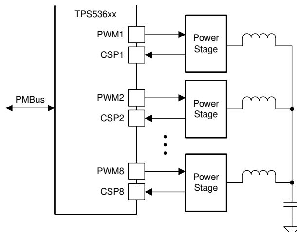
Simplified Schematic
