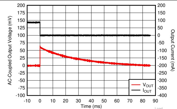
图 6-18. I_{OUT} Transient From 100 mA to 0 mA
