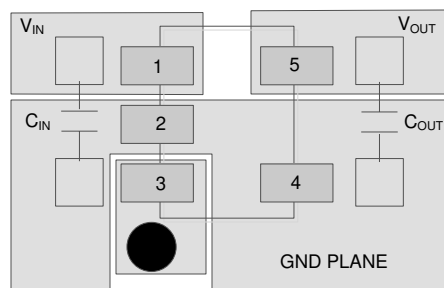
图 8-7. Layout Example for the DBV Package
