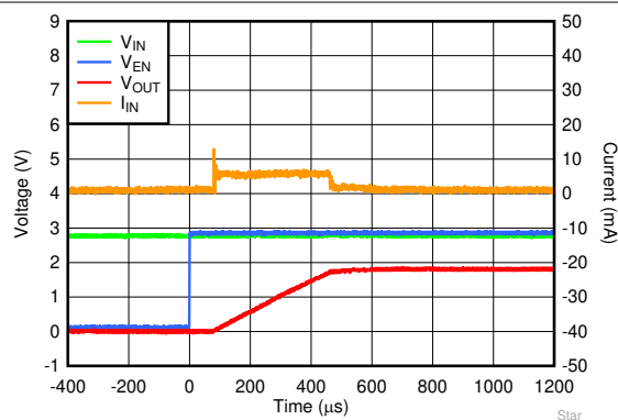
图 6-55. Startup Inrush Current With C_{OUT} = 1\text{ }\mu\text{F}
