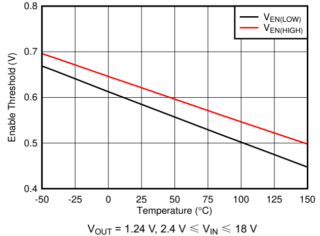
图 7-14. V_{EN} Thresholds vs Temperature
