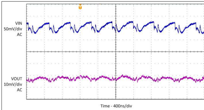
图 24. Input and Output Ripple in PWM Mode
