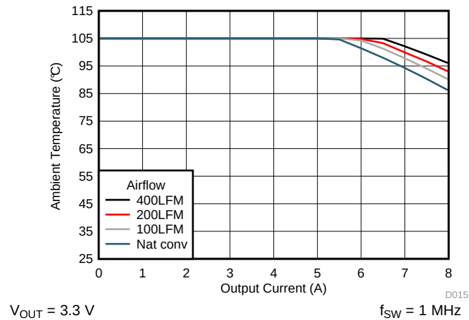
图 11. Safe Operating Area
