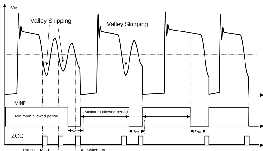
Figure 28. Valley Skipping
