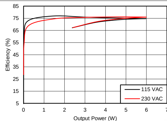
Figure 44. Efficiency vs P_{OUT} Diagram
