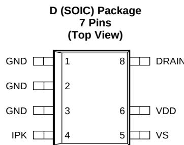
Pin Functions
