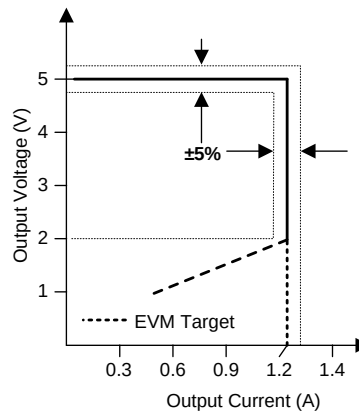
Figure 33. Target Output V-I Characteristic
