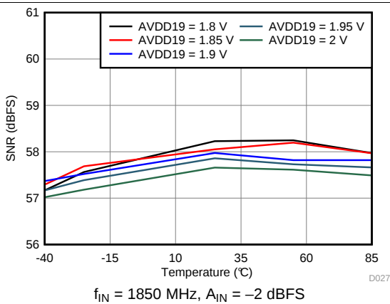
Figure 29. Signal-to-Noise Ratio vs AVDD19 Supply and Temperature
