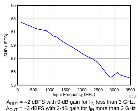
Figure 20. Signal-to-Noise Ratio vs Input Frequency
