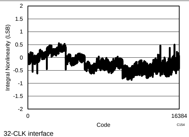
Figure 47. Typical INL
