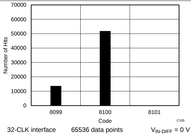
Figure 41. DC Histogram
