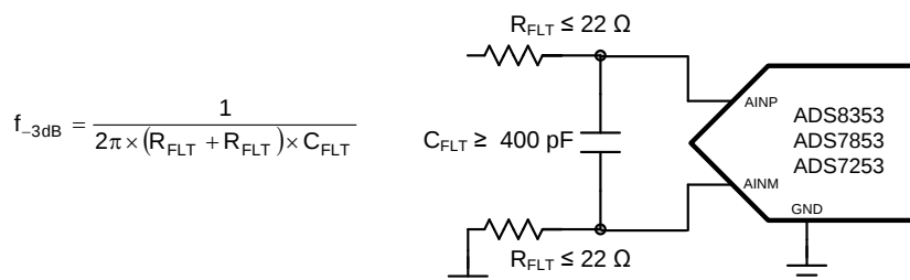
Figure 100. Antialiasing Filter
