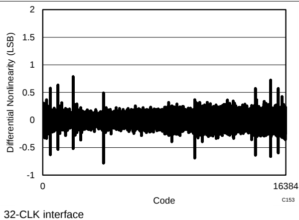
Figure 46. Typical DNL
