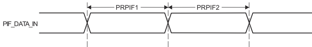
图 6-102. PRU_ICSSG PRU Peripheral Interface Timing
