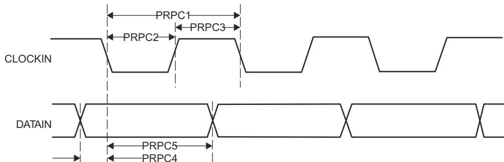
图 6-97. PRU_ICSSG PRU Parallel Capture Timing - Falling Edge Mode
