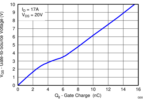
栅极电荷
